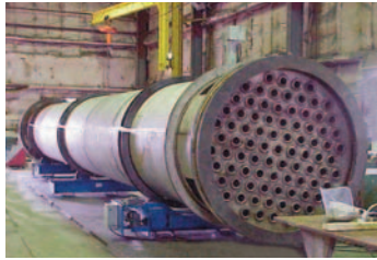
Air preheater
